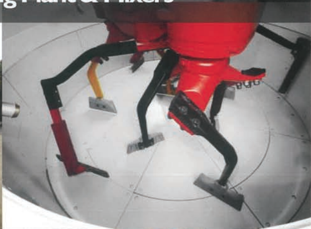
Batching Plant & Mixers
